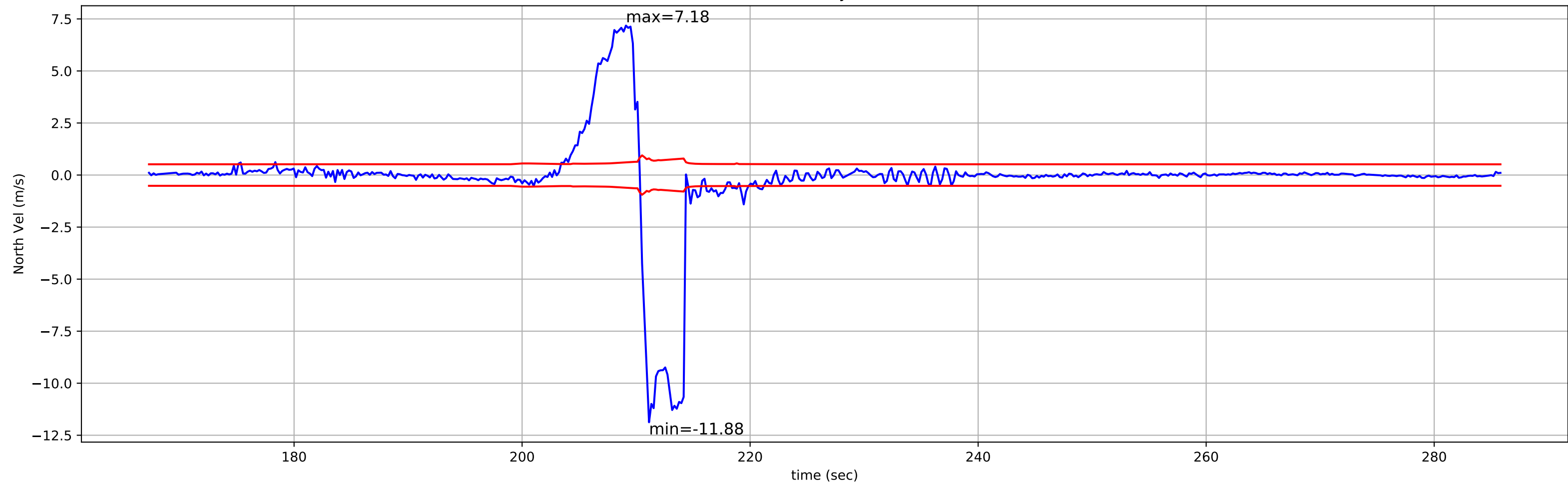
Horizontal Velocity Innovations
