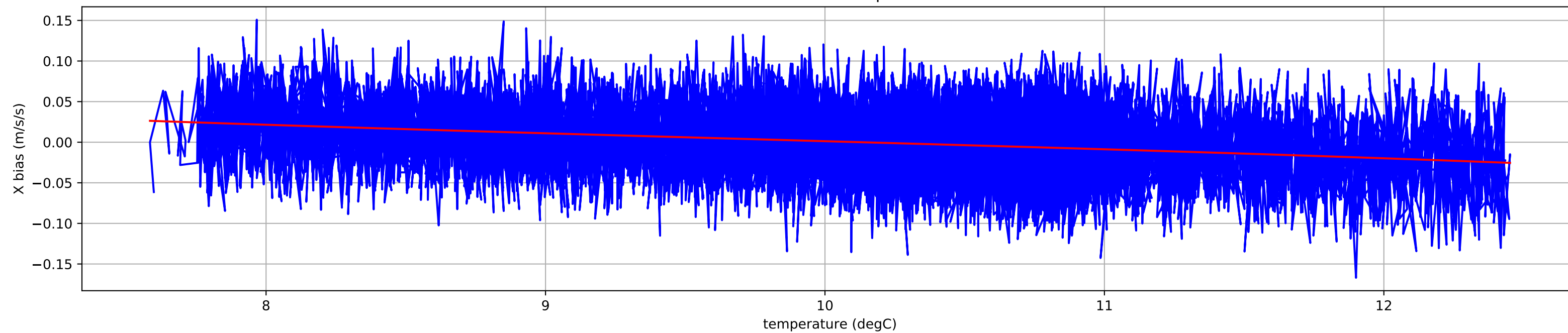
Accel 0 Bias vs Temperature
