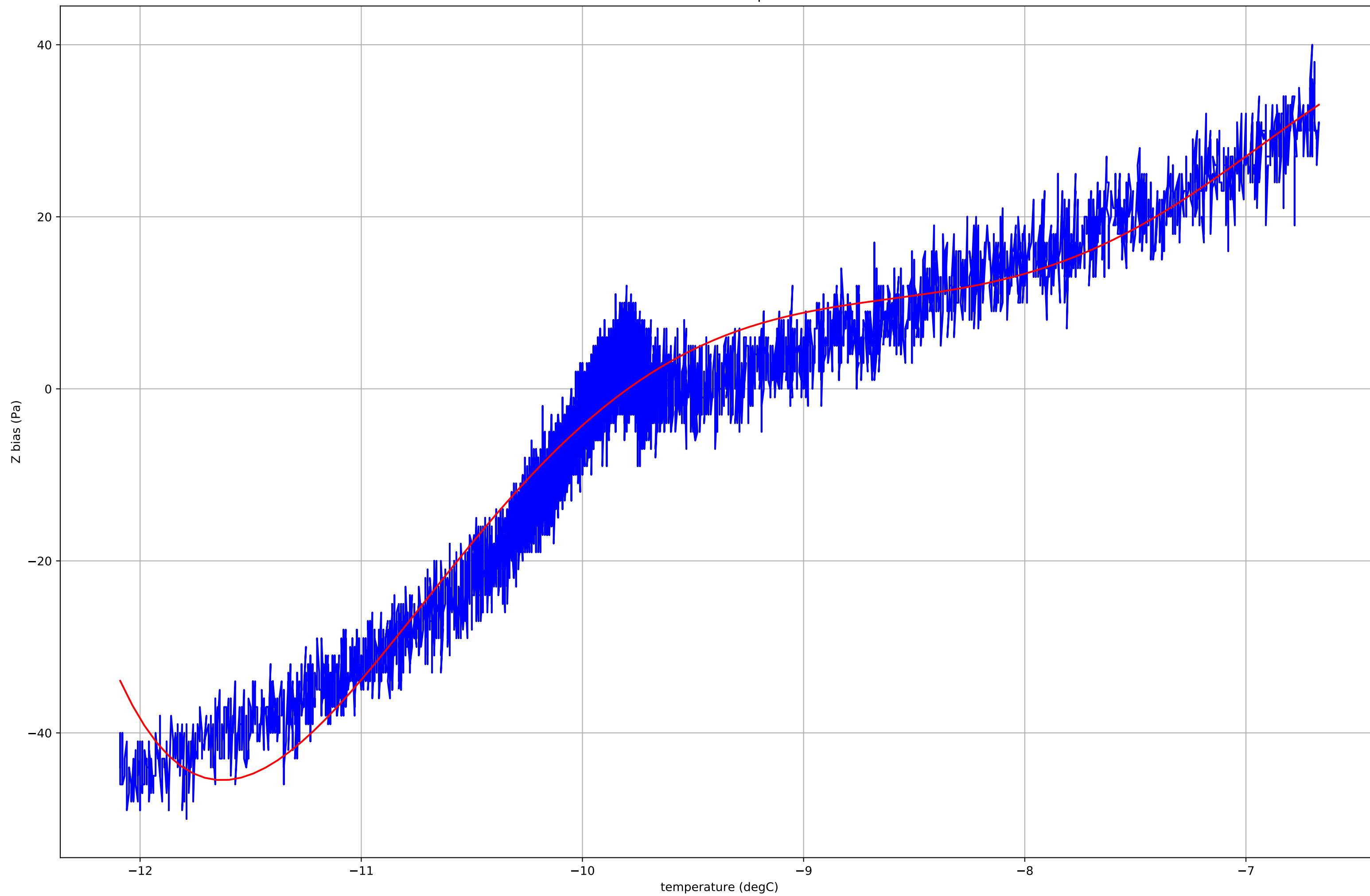
Baro 1 Bias vs Temperature
