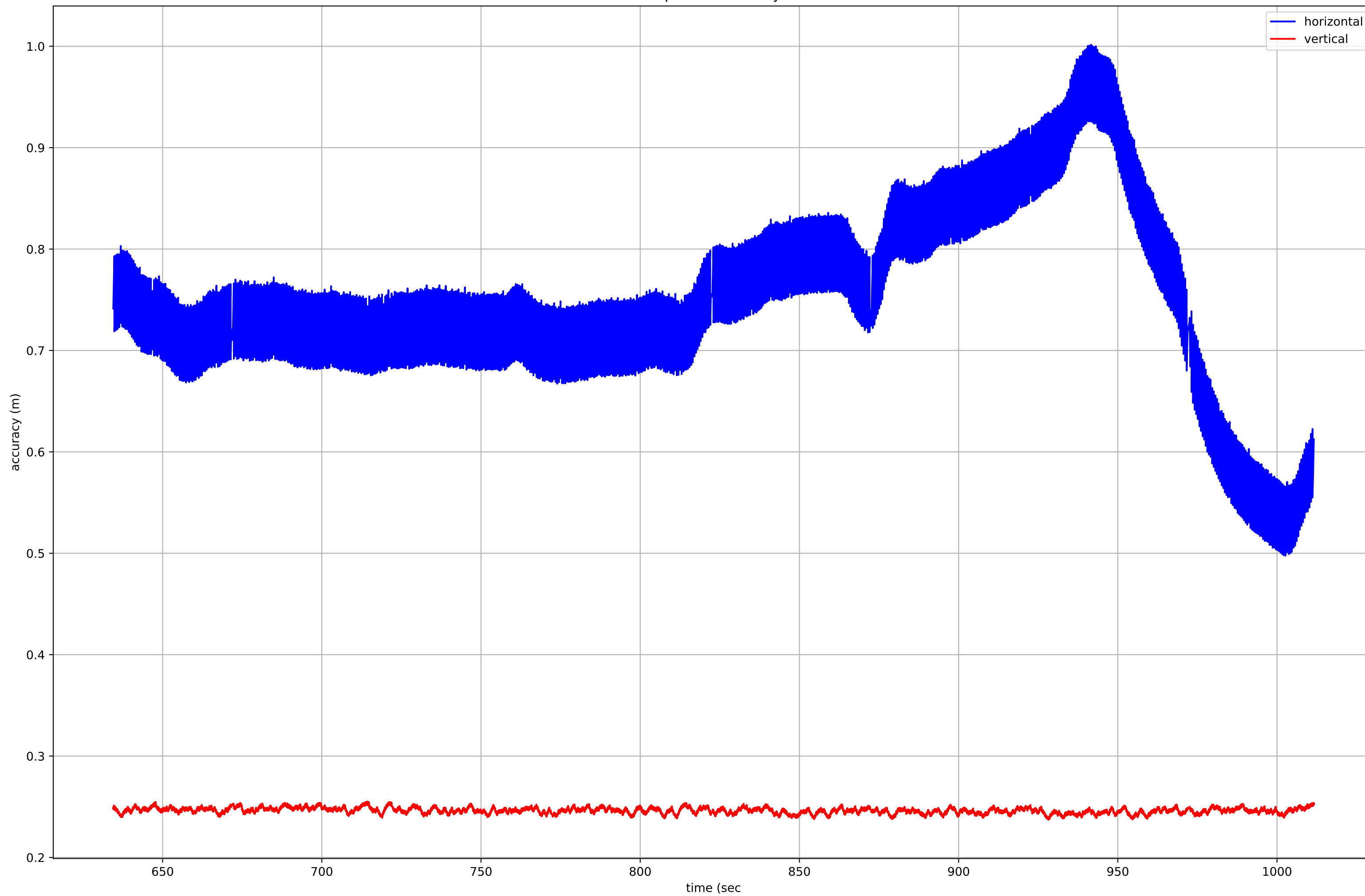
Reported Accuracy
