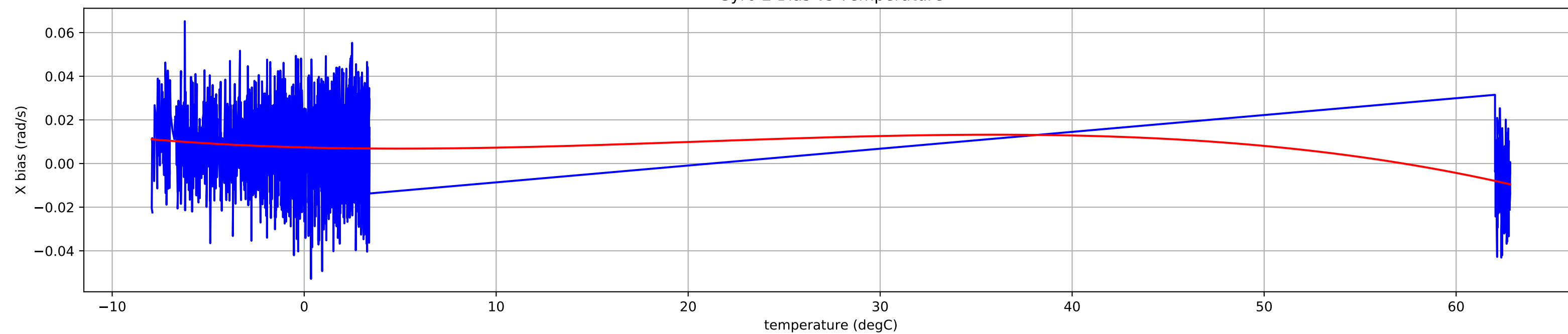
Gyro 2 Bias vs Temperature
