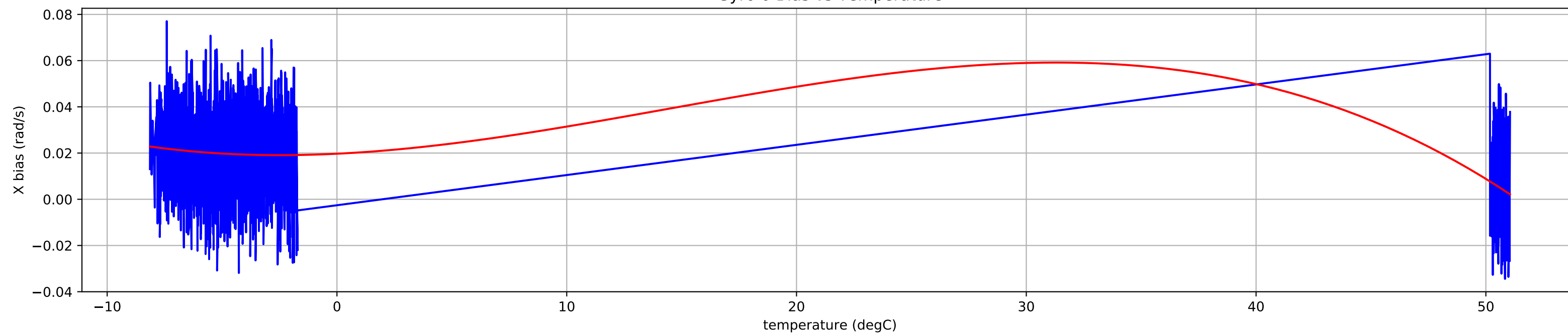
Gyro 0 Bias vs Temperature
