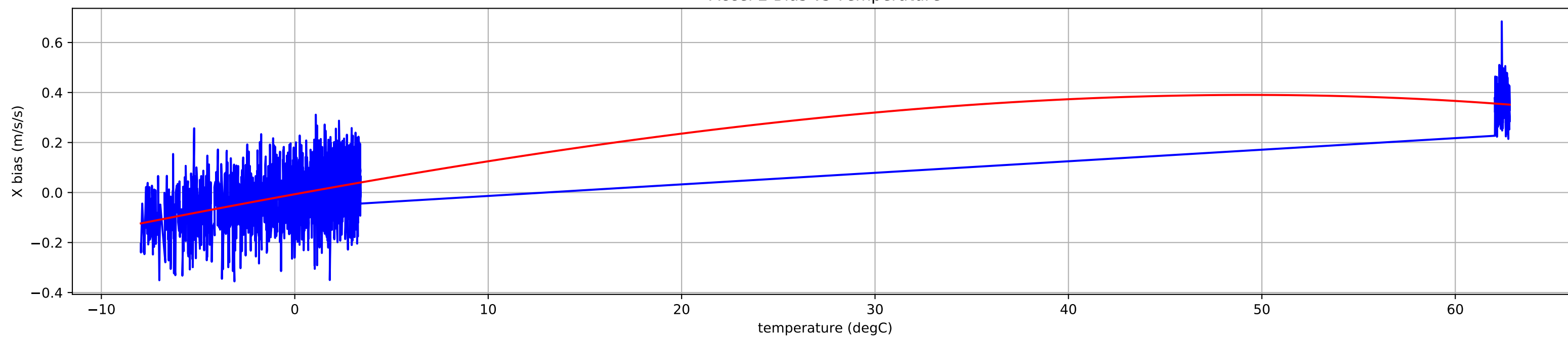
Accel 2 Bias vs Temperature
