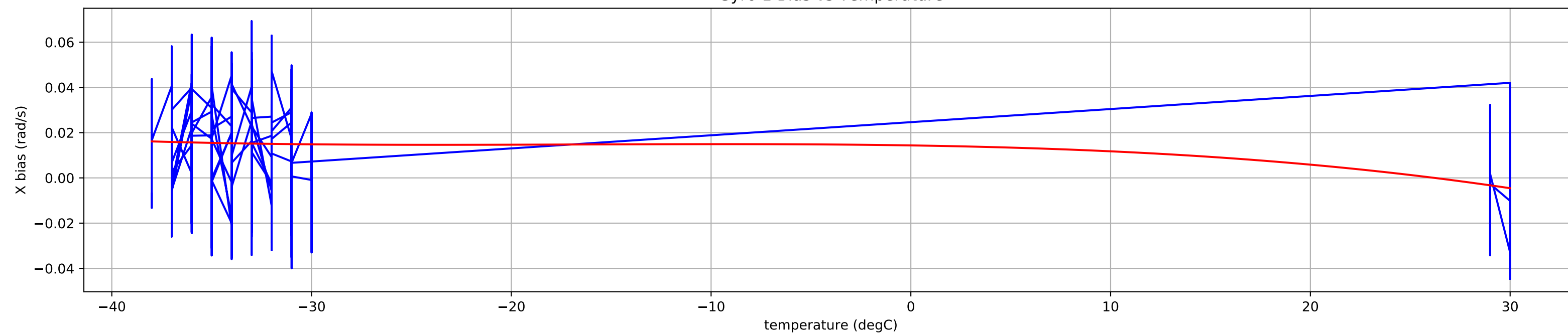
Gyro 1 Bias vs Temperature
