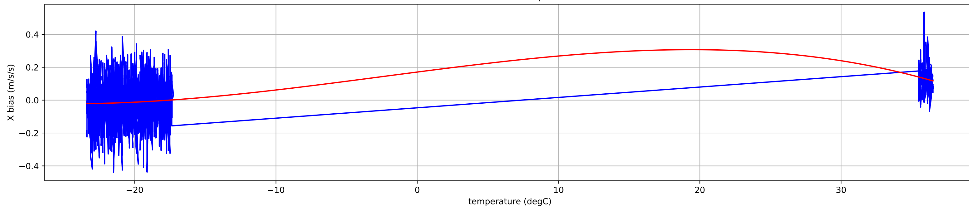
Accel 1 Bias vs Temperature
