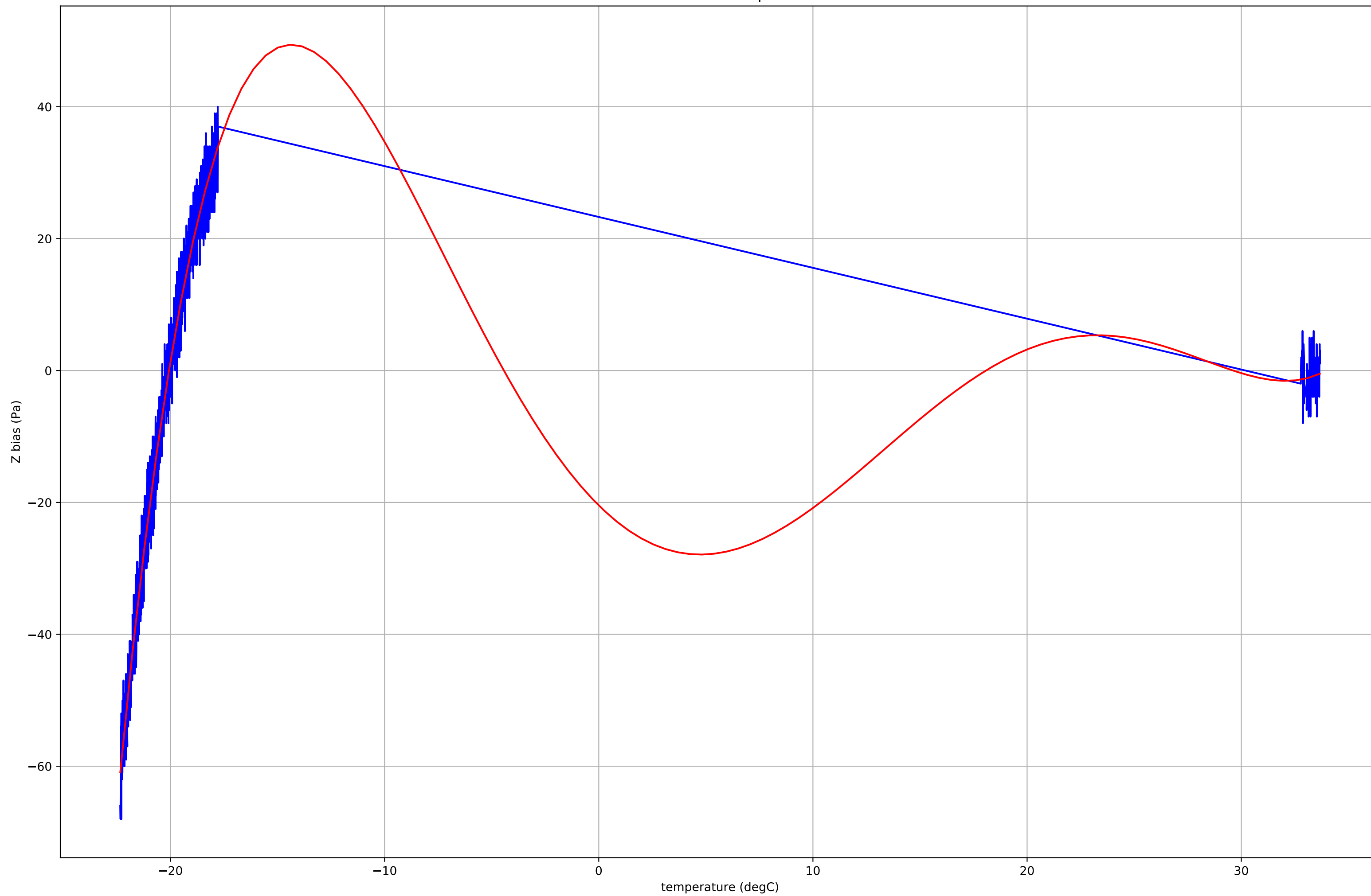
Baro 0 Bias vs Temperature
