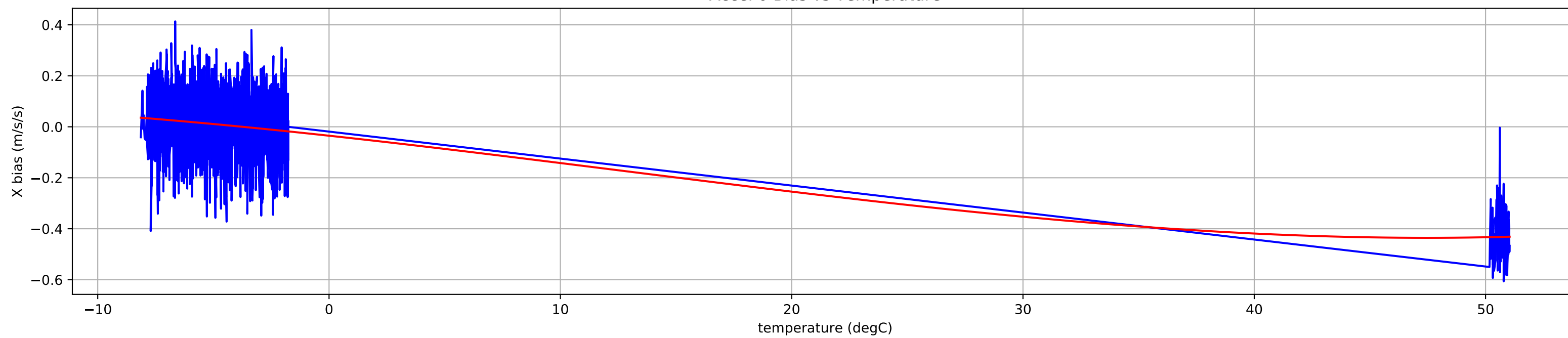
Accel 0 Bias vs Temperature
